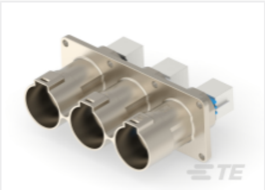
TE 产品编号2399608-1 3POS,HVP1400,ASSY,180DEG,COD A /B/C
