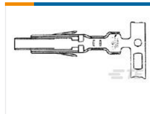
TE 产品编号170312-1 POWER CONN.CONTACT
