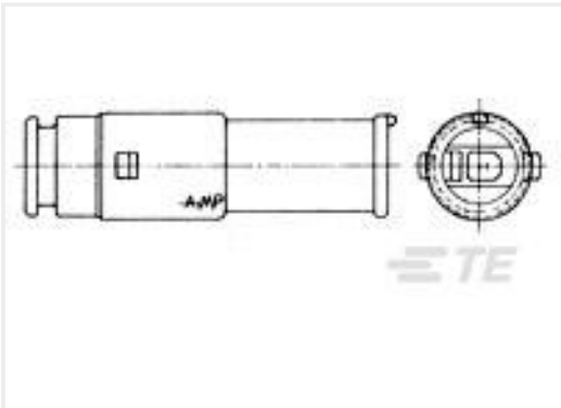
TE 产品编号172281-2 ECONOSEAL CONN CAP 12P
