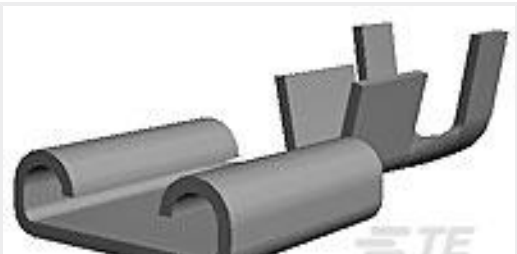
TE 产品编号170224-2 250 FASTON,REC.,16-10 AWG,BR
