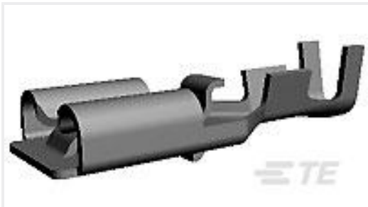
TE 产品编号179975-1 250 PL EX REC. 15-10AWG PTBR
