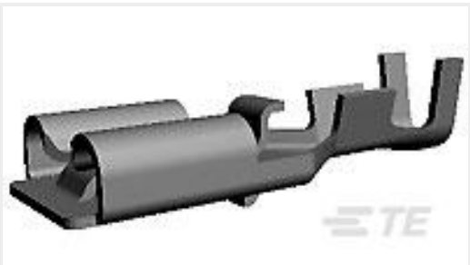
TE 产品编号179973-1 250 PL EX REC. 22-18AWG PTBR
