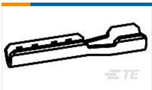
TE 产品编号62382-1 SPLICE 25/26 .012 BR
