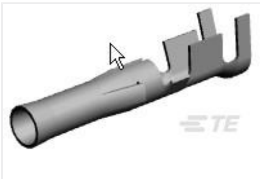
TE 产品编号770144-1 .093 CP&S SOK PTPBR L/P 20-14
