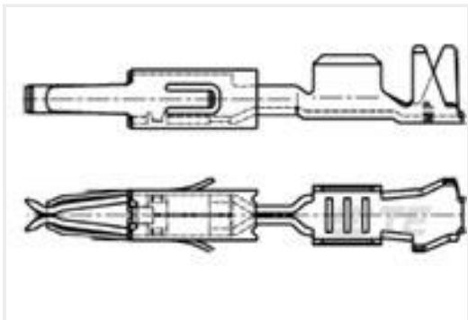
TE 产品编号964274-2 MT2 A REC 1.6 Contact SWS Sn
