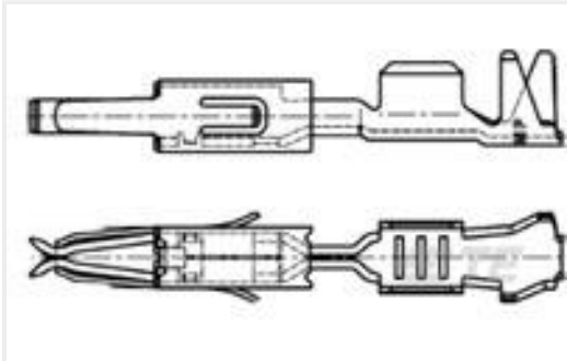
TE 产品编号964274-2 MT2 A REC 1.6 Contact SWS Sn
