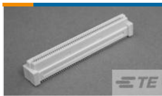
TE 产品编号5-5179009-3 0.8FH,R09H.5,080,08/Sn,TU
