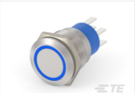
TE 产品编号5-2213767-7 AV19 DPM 3A MOVE RING LED BLUE 12V
