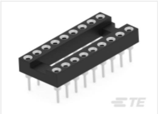
TE 产品编号2485264-5 DIP IC SOCKET 18P, Sn
