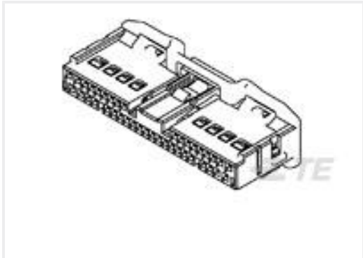
TE 产品编号1827842-1 0.50 SERIES CONN 40POS PLUG ASSY TYPE-A
