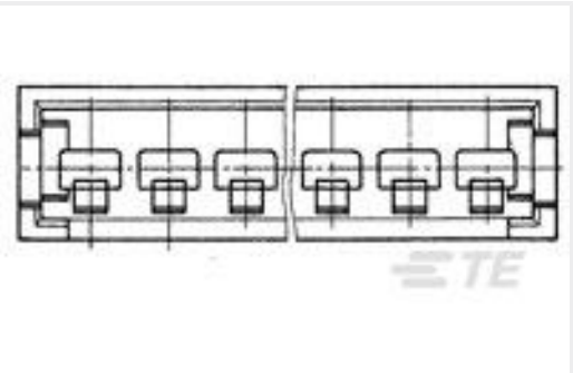
TE 产品编号280631 AMPMODU II COSI PIN HSG, SGL ROW, 8 POS.
