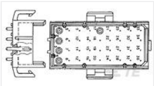
TE 产品编号640504-1 20P MR HDR ASSY V0
