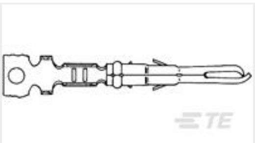
TE 产品编号640545-1 MR SPLIT PIN 26-18 PTPHBRZ LP
