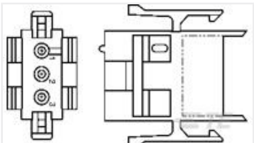
TE 产品编号1-640508-0 03P MR II CAP HSG V0
