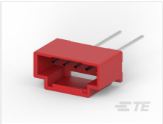
TE 产品编号5-2232546-3 GI2.5 HDR ASS 5P RED NO BOSS TAPE
