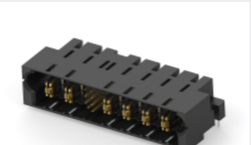
TE 产品编号5-6450840-4 MBXLE R/A HEADER 2ACP + 8S + 4ACP
