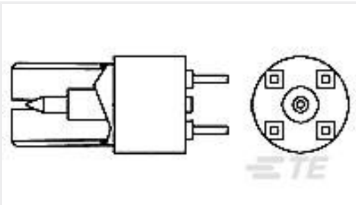
TE 产品编号1274531-1 N SERIES, SURFACE MOUNT PCB
