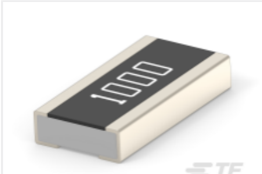
TE 产品编号2-2176558-8 3430 B2 1% 12R 100ppm 1k RL
