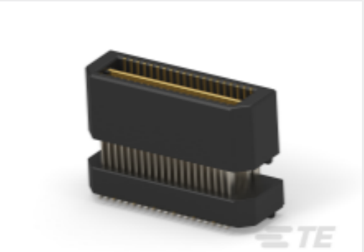
TE 产品编号 4-1658438-1 MSB0.80PL14ASY040FL,GP,10,-TR
