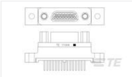
TE 产品编号1532267-3 M83513/22-B01NN = MCKS-N1-B-15PST1
