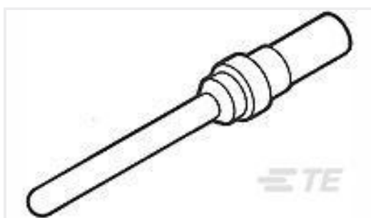
TE 产品编号1218266-1 CONT, CRIMP PIN, 18AWG, 109, SZ 20
