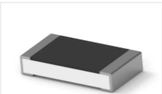
TE 产品编号2-2176389-7 RQ 1206 200R 0.1% 10PPM 5K RL
