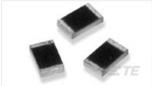
TE 产品编号9-1879261-1 RP 2B 12K1 0.1% 15PPM CUT LENGTH
