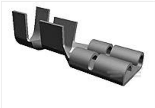
TE 产品编号63757-2 250 FASTON REC 16-12 AWG NPST 247 E
