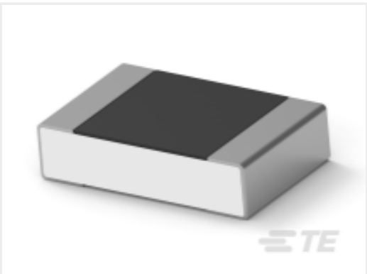
TE 产品编号7-2176373-2 RQ 0805 54R9 0.1% 10PPM 1K RL
