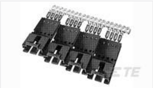
TE 产品编号5-103945-5 2X6 MTE SHRD PIN SR LATCH .100
