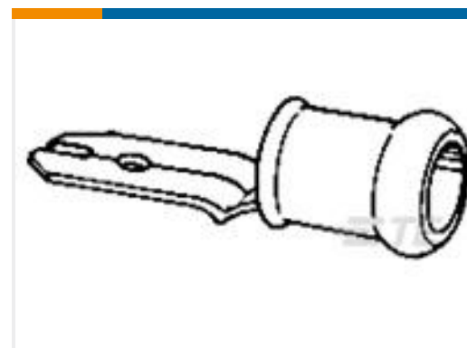
TE 产品编号141085-2 TERMINAL TAB FASTON PIDG 6,35
