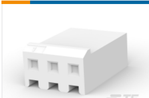
TE 产品编号647402-7 Receptacle Housing: Wire-to-Board, with Mating Alignment, SL156
