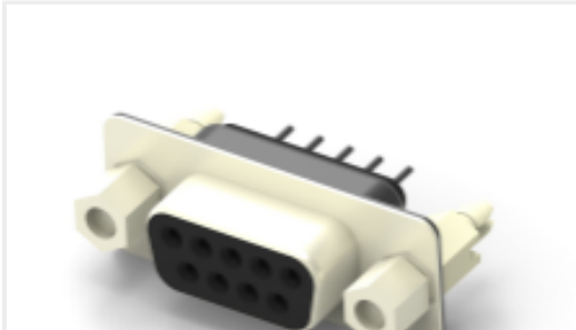
TE 产品编号2301838-2 AMPL REC HD20, VERT, 9P, B/L,4-40 S /LOCK
