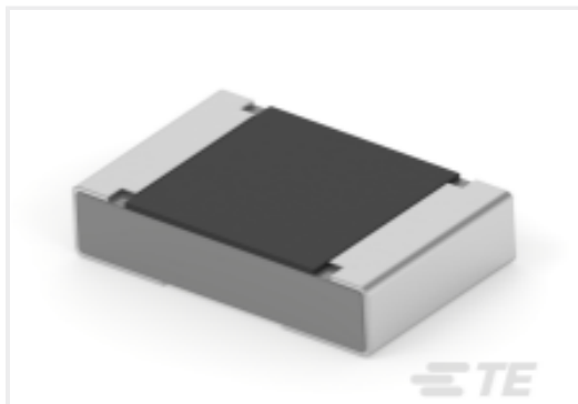
TE 产品编号4-2176477-8 RA73F 2A 1K69 0.1% 1K RL
