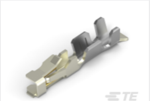
TE 产品编号5-2316114-6 2MM,REC,CNT,CRIMP,28-30AWG,0.76 UM,LP
