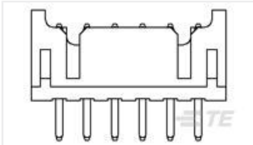
TE 产品编号1470109-6 2.0mm Pitch Header,Dip 6p
