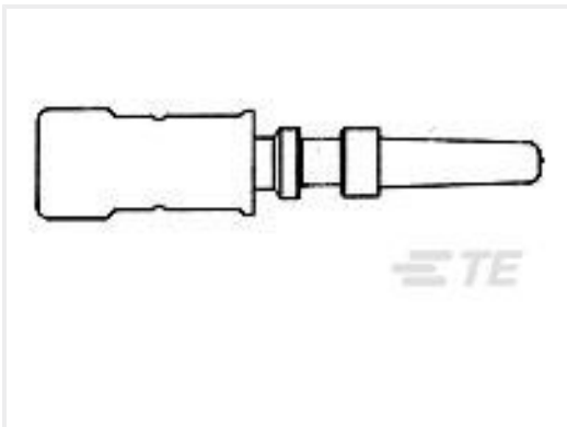
TE 产品编号42574-3 PIDG, TAPER PIN
