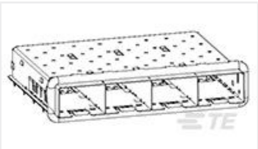
TE 产品编号2198722-1 CAGEASSY, PRESSFIT, 1X4, zSFP+
