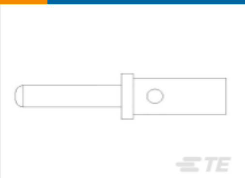
TE 产品编号JN1003P22D CONTACT PIN. #22
