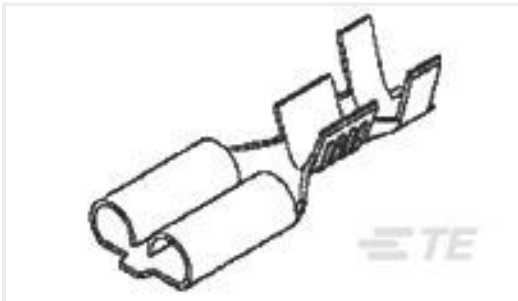
TE 产品编号170384-2 250 FASTON,REC.,22-20 AWG,TPBR
