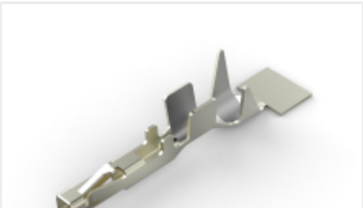
TE 产品编号2008625-2 Socket Micro MNL, GOLD 22-18
