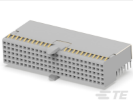
TE 产品编号3-646547-0 Z-PACK A-B 25 COLUMN SHLD ASSY
