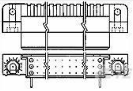
TE 产品编号532431-3 HDI RECP ASSY 3 ROW 96 POS
