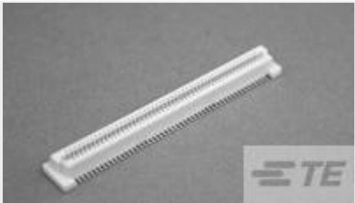
TE 产品编号2-1735481-1 0.8FH,R17H.5,040,30/Sn,TU,SC
