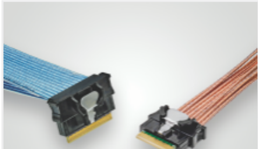
TE 产品编号2821376-1 SLIVER C/A, 74P, STR TO STR, 25GHZ 85OHM
