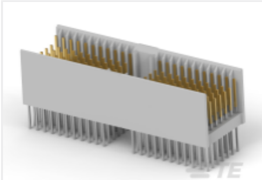
TE 产品编号5188399-9 Z-PACK/A M-HDR 154P
