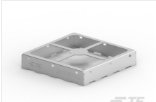
TE 产品编号2118718-2 STD SHIELD FRAME, CRS-26.21X26.21X5.08MM
