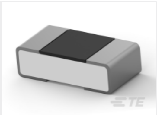
TE 产品编号5-2176364-0 RQ 0402 15K 0.1% 10PPM 5K RL
