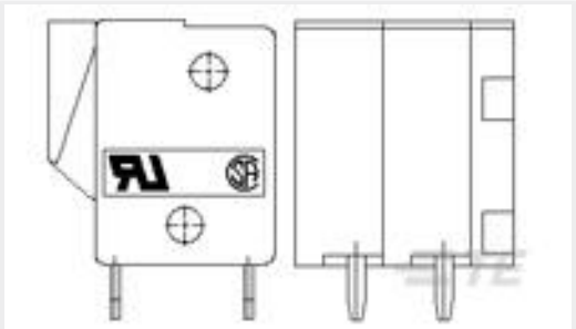
TE 产品编号1776259-8 8P Spring TB, 180deg, VT,5mm, Green
