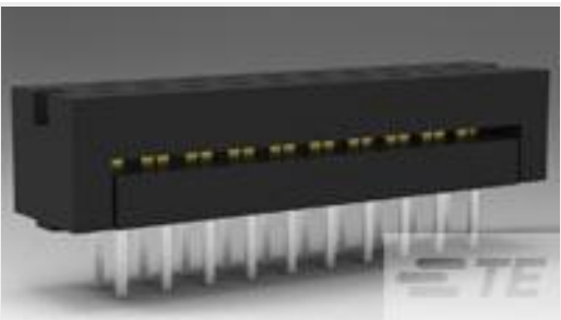
TE 产品编号746610-8 034 DIP PLUG 100CL TIN
