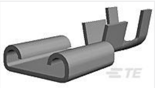
TE 产品编号170187-2 250 FASTON,REC.,22-18 AWG,TPBR
