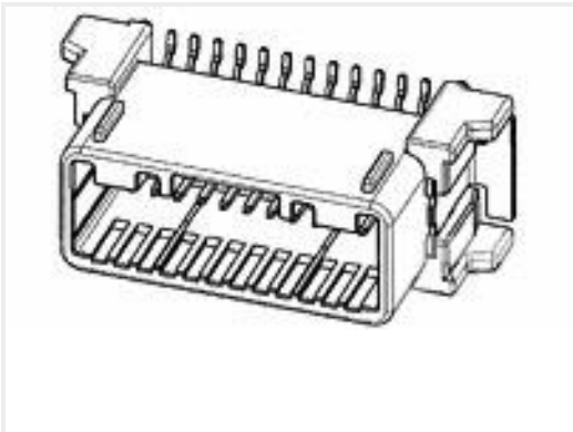
TE 产品编号1717394-2 0.64 SMD 24POS CAP ASSY V TIN
