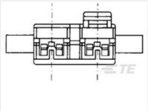
TE 产品编号353253-1 PL EX 110 (2.8 MM) HOUSING RECEPTACLE
