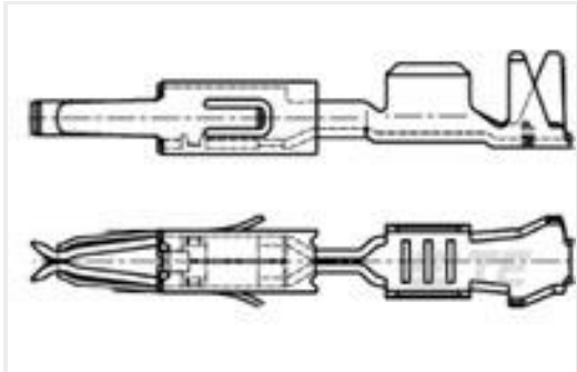
TE 产品编号964261-2 MT2 A REC 1.6 Contact SRC Sn
