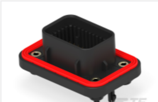
TE 产品编号2388688-1 34POS,PIN DIA 1.0,HDR ASSY,180DEG
