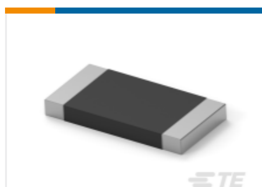
TE 产品编号3-2176421-2 TLRP 2512 2.0W R075 1% 25PPM 4K RL
