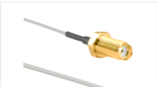
TE 产品编号CSI-SGFB-200-UFFR SMA to U.FL/MHF1 200mm 1.13 OD
