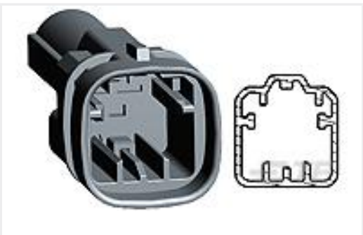
TE 产品编号1544606-1 TAB HOUSING, 8MM NG1, 1 WAY
