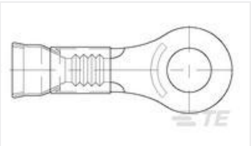
TE 产品编号150492 TERM, RT,STRAT,DGRP, HR, 22-16, M3.5(#6)
