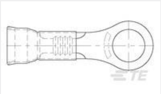
TE 产品编号1958447-1 STRATO-THERM,DG,RT,HR,26-22 AWG,#2, NI
